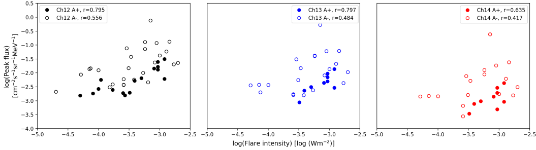
Figure 1. Plot of the logarithm of the flare intensity versus logarithm of the proton peak flux for the three high energy GOES channels. The y-axes span equal orders of magnitude. A+ and A- events are shown as filled and empty circles respectively. Black, blue and red circles correspond to events in Ch12, 13 and 14 respectively (left to right panels). Correlation coefficients, r , for each group are labelled.
