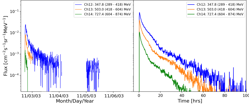
Figure 2. Comparison of the forecast flux profile in Ch 12, 13 and 14 from SPARX–H (right) and the calibrated and background subtracted dataset from GOES observations (left) for the GLE event of 2 November 2003. Both observed and forecast profiles are shown for a period of 100 hours following the flare.
