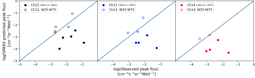
Figure 3. The observed and SPARX–H predicted logarithm of the peak fluxes for the historic test SEP events over the three high energy channels. Unfilled circles show events with associated flare longitudes between W25 and W75. The blue line is the 1:1 line.
